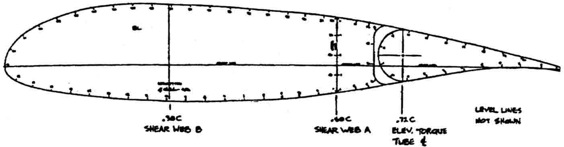
CANARD LS(1)0417Mod AIRFOIL
